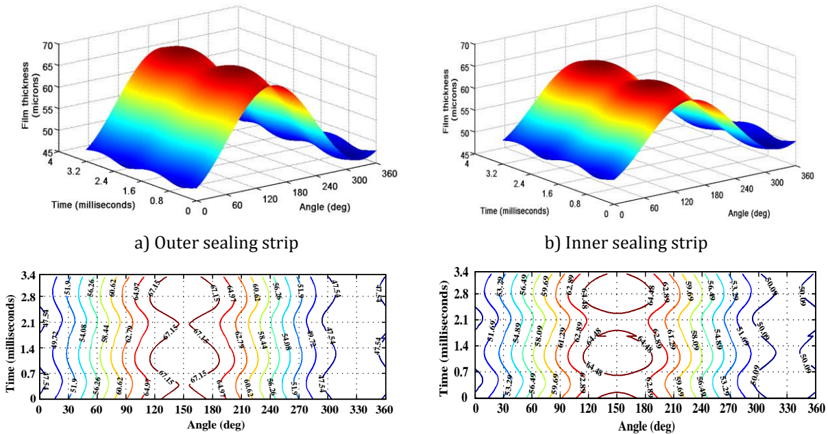
c) Oil film thickness distribution of outer sealing strip
